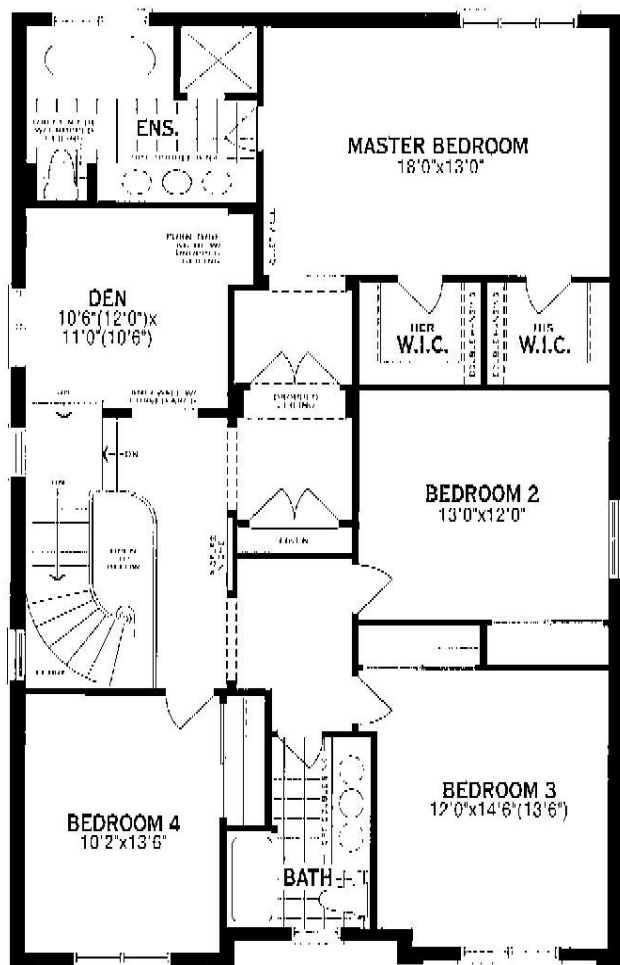
SECOND FLOOR PLAN 4 BEDROOM & DEN
